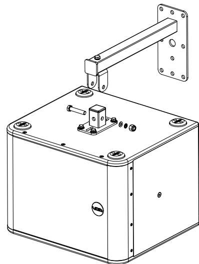
Figure 5.40: Loudspeaker fixing
