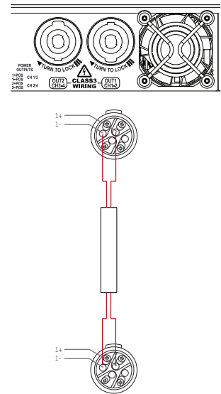
Figure 4.11: Bias Q3/Q5 speakON™ wiring
