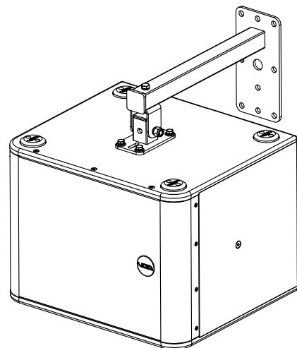
Figure 5.40: Loudspeaker fixing
