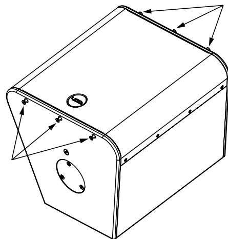
Figure 5.31: Grille removal
