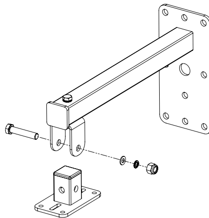
Figure 5.37: Nut removal
