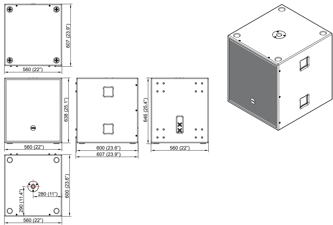
Figure 4.1: Dimensions
