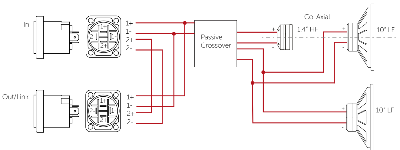
Figure 4.1: Airten V3 wiring diagram
