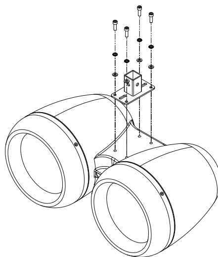
Figure 5.18: T75 attachment
