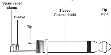
Unbalanced use of 1/4" jack TS connector
