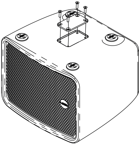
Figure 5.9: Bolt removal
