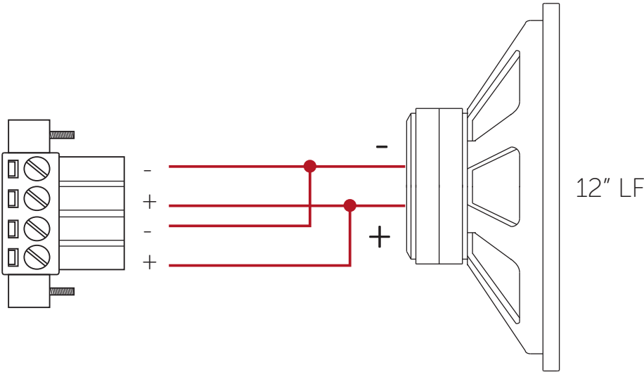
Figure 4.6: Wiring diagram
