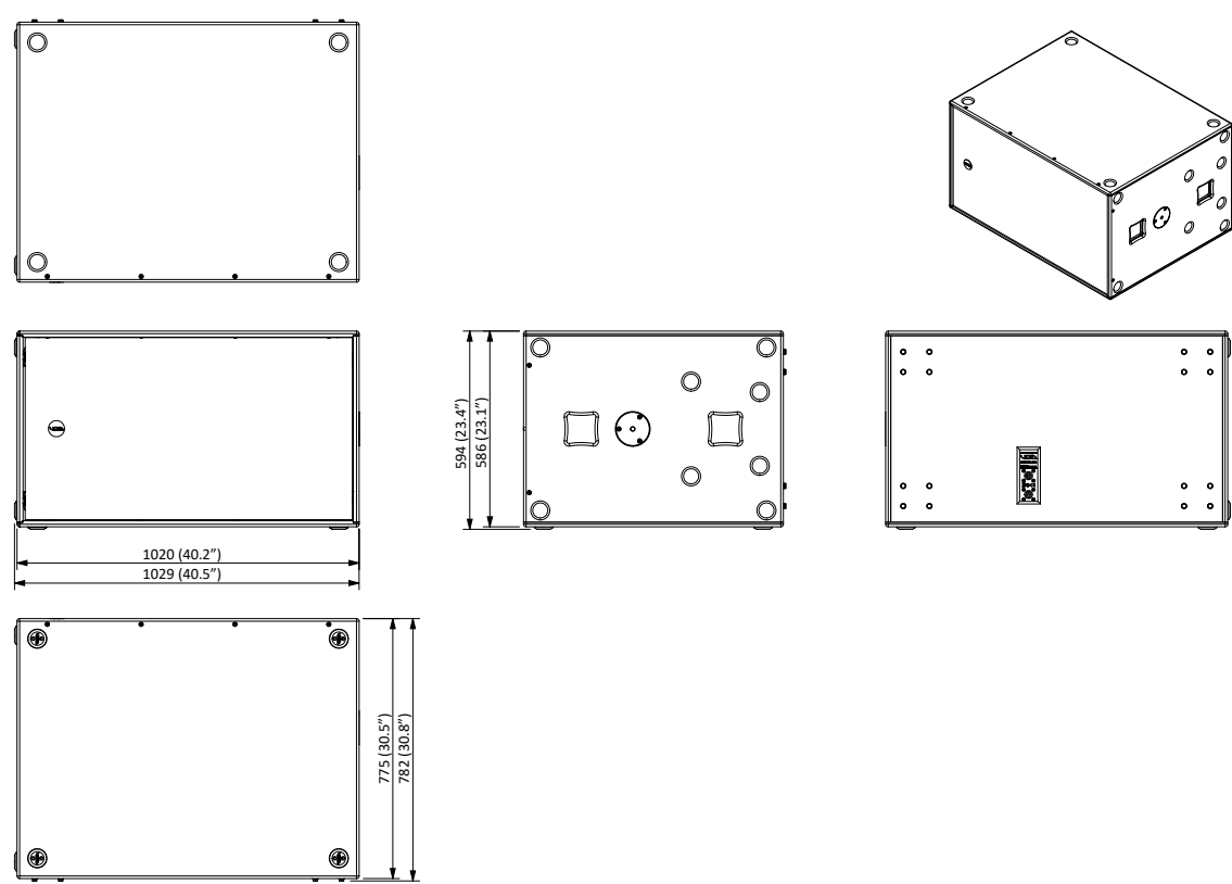
Figure 4.1: Dimensions
