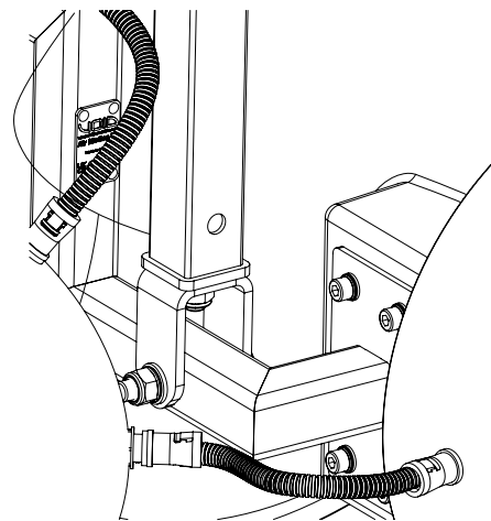
Figure 5.24: Safety wire attachment
